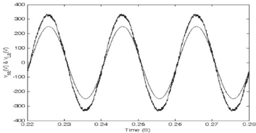
Fig 7: Voltages at the PCC and load terminals.
