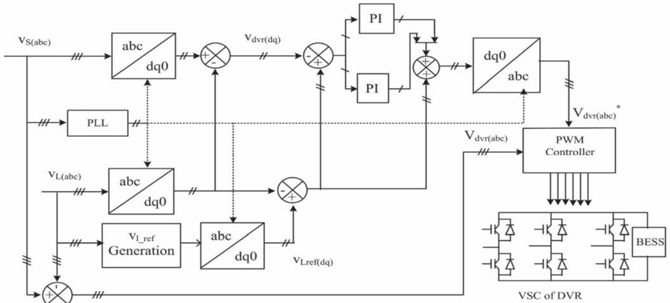
Fig 3: Control block of the DVR that uses the SRF method of control.
