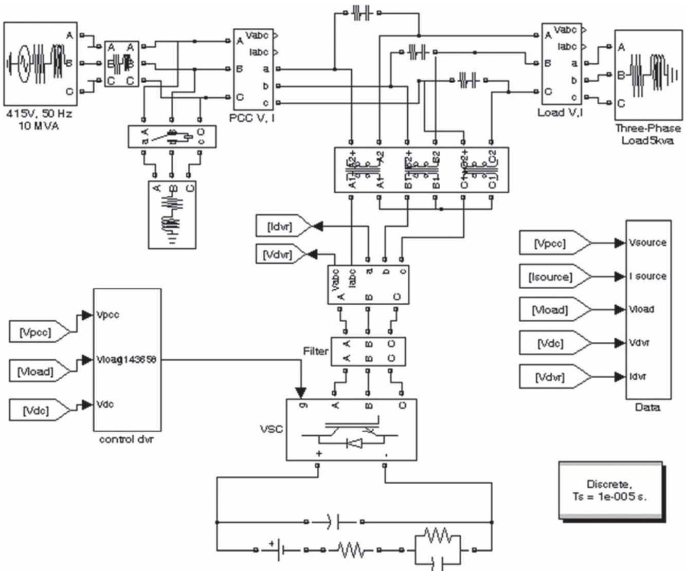
Fig 5: MATLAB-based model of the BESS-supported DVR-connected system.
