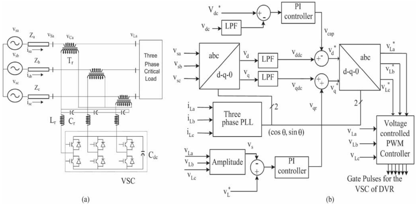
Fig 4(a): Schematic of the self-supported DVR. (b) Control block of the DVR that uses the SRF method of control. The reference DVR voltages are obtained in the rotating reference frame as
