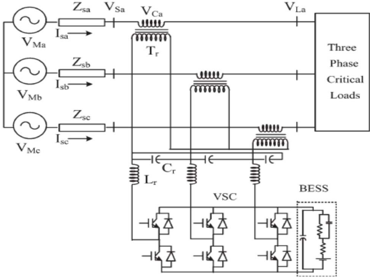
Fig 2: Schematic of the DVR-connected system.
