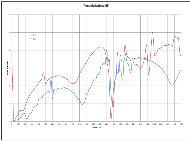
Fig 10: Comparison of transmission loss between both geometries.
