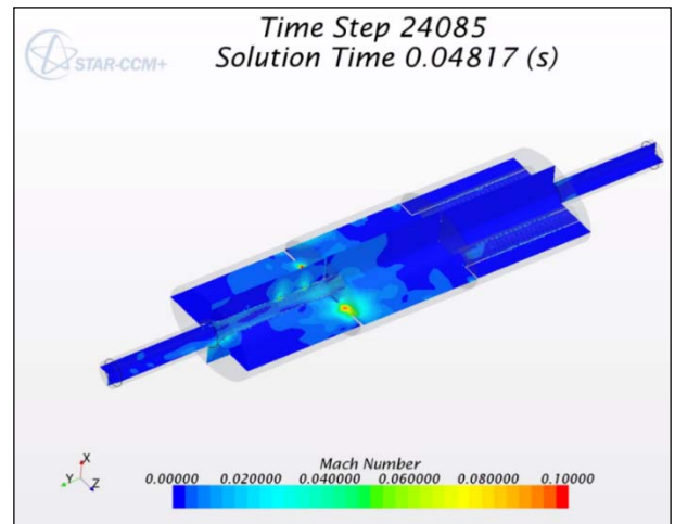
Fig 7: Velocity distribution inside the muffler
