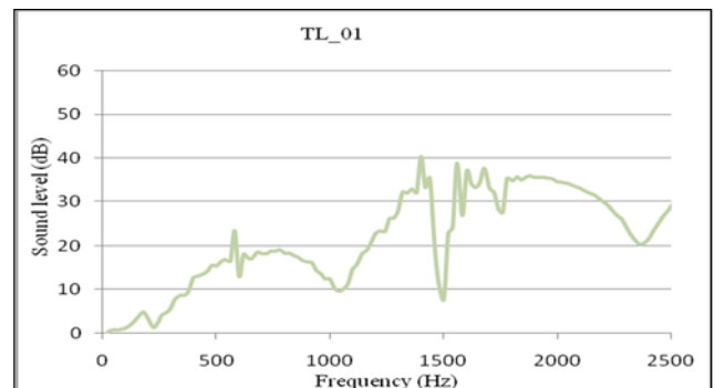
Fig 8: Transmission loss of Geometry-1
