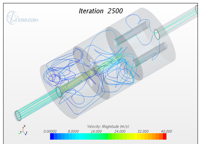
Fig 15: Velocity Streamlines for Geometry-2
