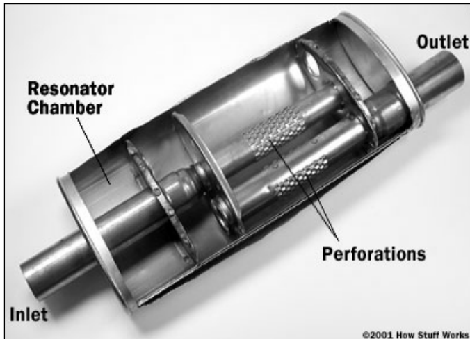
Fig 1: Typical reactive automotive muffler
