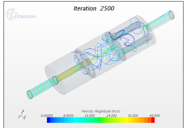
Fig 13: Velocity Streamlines for Geometry-1
