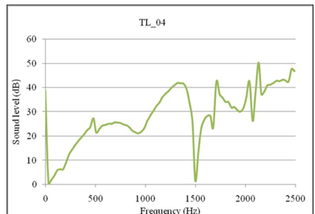
Fig 9: Transmission loss of Geometry-2
