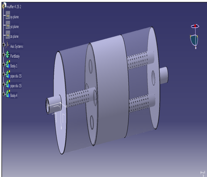
Fig 5: 3D CAD model of reactive muffler (Geometry -2)
