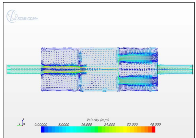
Fig 14: Velocity Contours for Geometry-1
