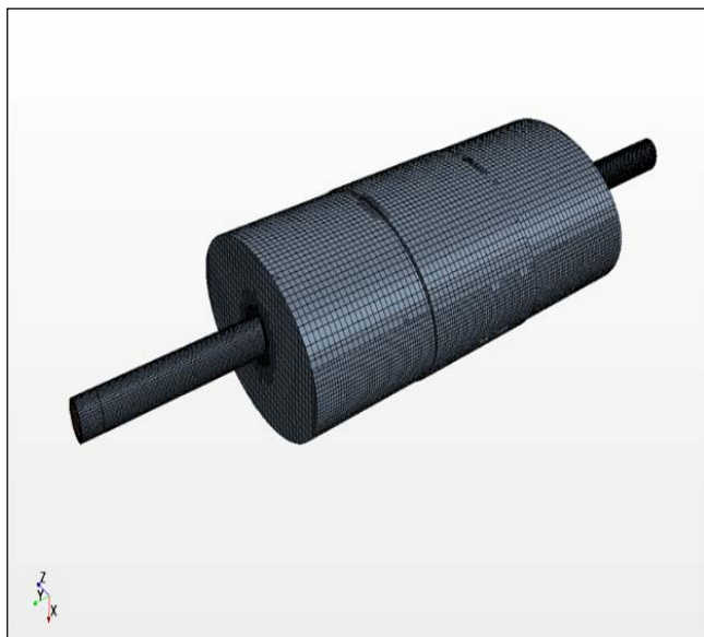
Fig 6: Mesh model
