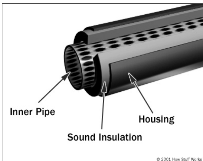
Fig 2: Typical absorptive automotive muffler
