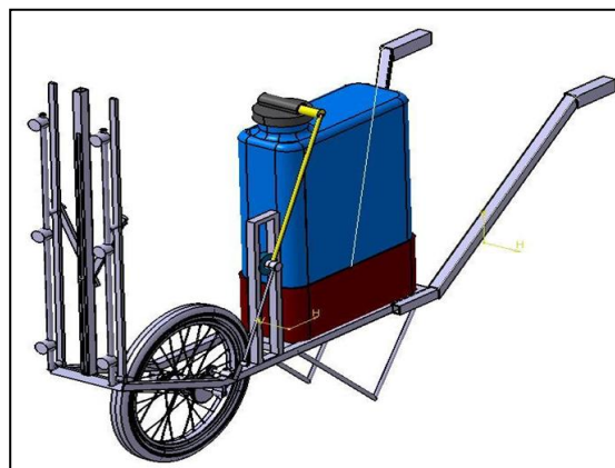
Fig 1: CAD model of manually operated multi-nozzle sprayer pump
